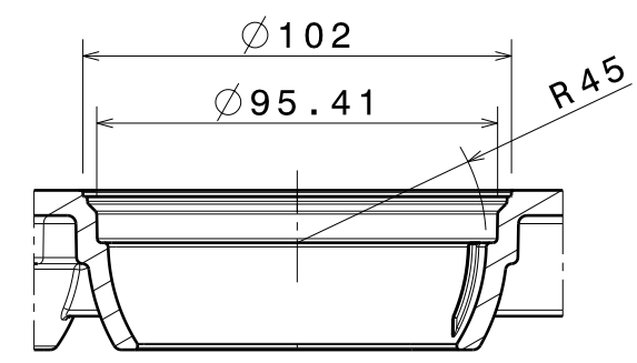
Section view C-C Scale: 1:2
